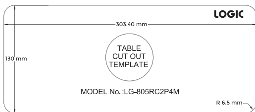
B: Cut-out template
