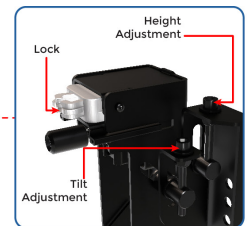
Multi- Dimensional Micro Adjustment Enables precision alignment of the video wall configuration including depth, height and tilt.
