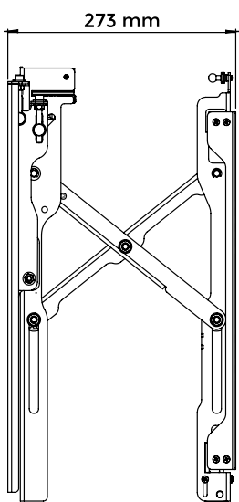
Side view When Opened
